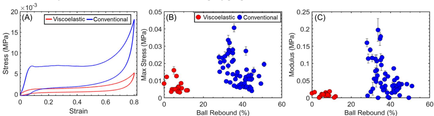
Figure 4: (A) Representative stress-strain curves. Similar curves were obtained for 45 foam samples. The (B) maximum stress (indicating resistance to deformation), and (C) the compression modulus of those foam layers were calculated as a function of rebound resilience values.
