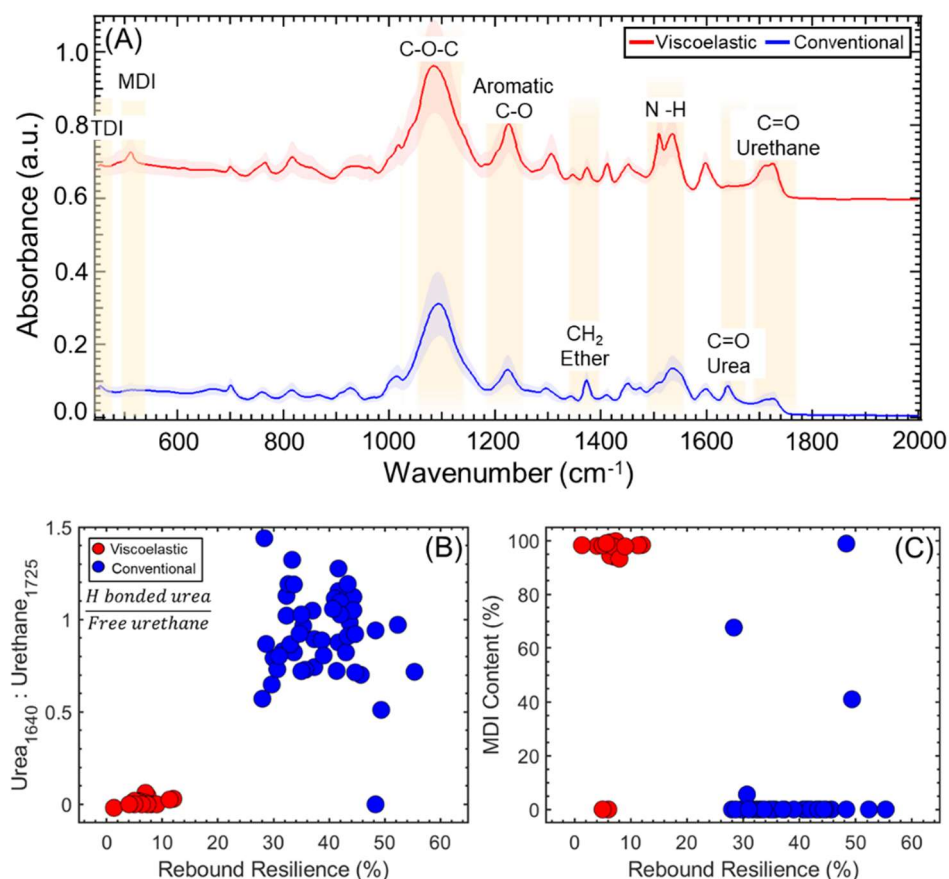
Figure 6 (A) FTIR spectra of viscoelastic and conventional foams were obtained. Ratios of absorbances of the (B) bidentate H-bonded urea and free urethane, and (C) MDI content were obtained from the FTIR spectra for both categories of foams.
